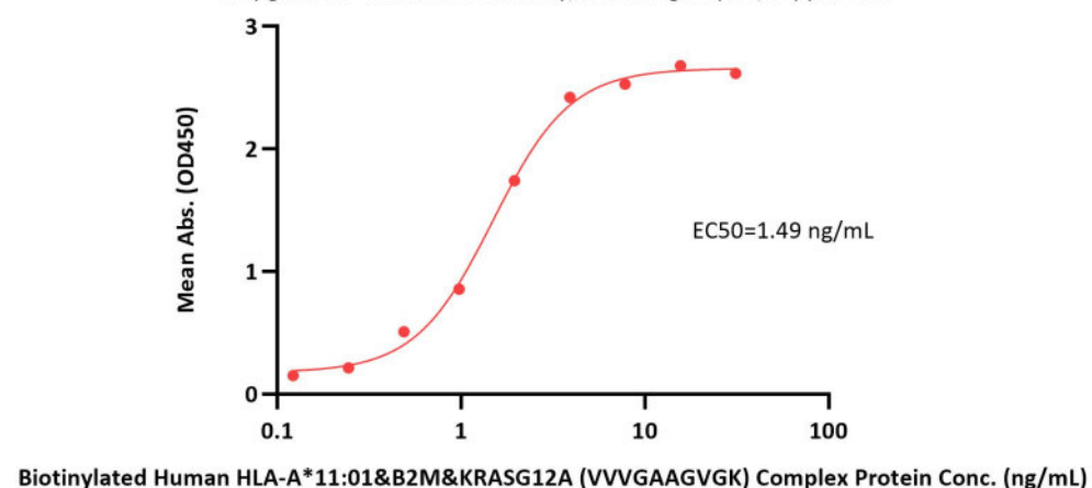
Biotinylated Human HLA-A*11:01&B2M&KRASG12A (VVVGAAGVGK) Complex Protein ELISA 0.1 µg of Anti-HLA class I Antibody, Human IgG1 (W6/32) per well
