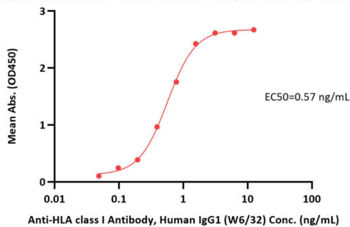
Biotinylated Human HLA-A*11:01&B2M&KRASG12A (VVVGAAGVGK) Complex Protein ELISA 0.1 µg of Biotinylated Human HLA-A*11:01&B2M&KRASG12A (VVVGAAGVGK) Complex Protein per well
